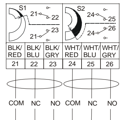
Figure 9: Auxiliary Switch Wiring Diagram for ES89Ax-S Series Models
