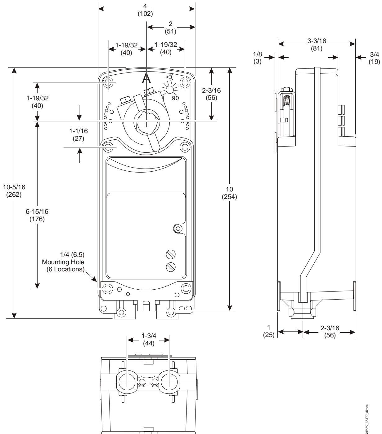
Figure 1: ES89Ax(-S) Series On/Off Electric Spring Return Actuator Dimensions, in. (mm)
